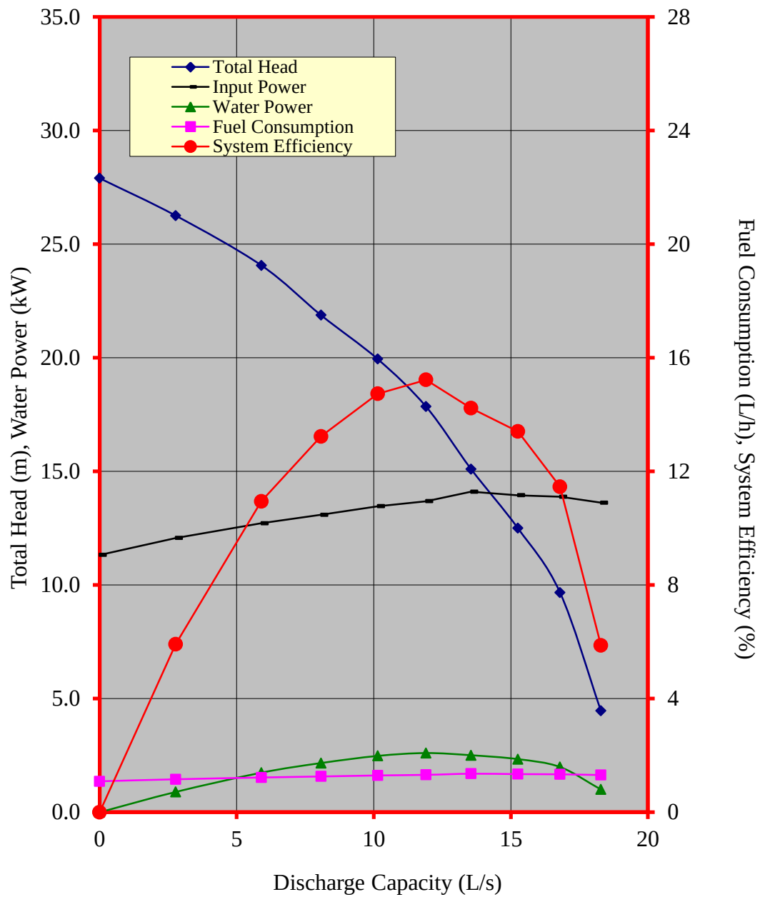
Figure 3. Performance characteristic curves of the KAMA KDP40 self-priming centrifugal pumpset
